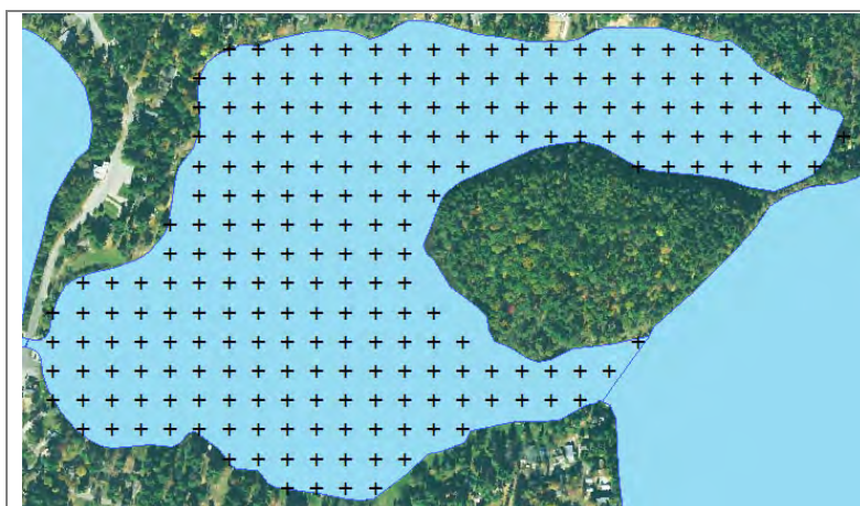
Figure 8.2.2-1. Grass Lake whole-lake aquatic point-intercept survey sampling locations.
