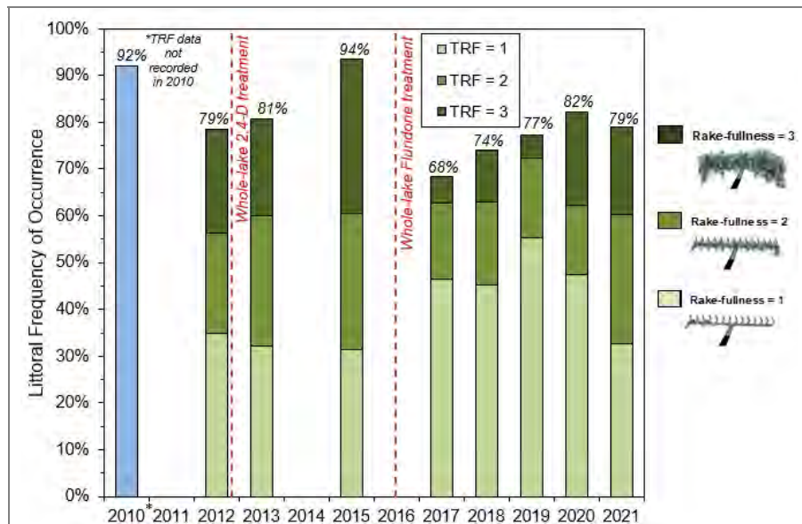
Figure 8.2.2-2. Total rake fullness ratings on Grass Lake. Created using data from point-intercept surveys.
