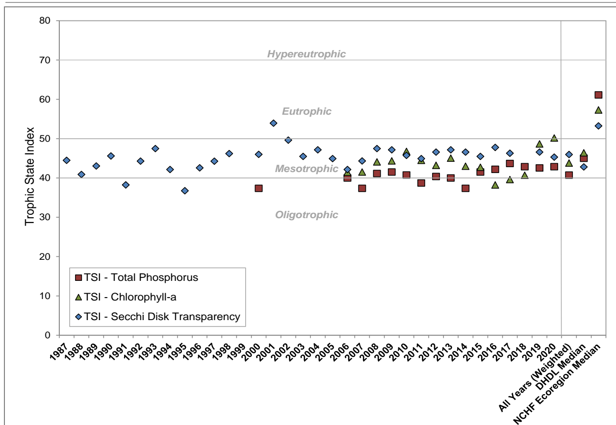
Figure 8.2.1-5. Grass Lake, state-wide deep headwater drainage lakes, and regional Trophic State Index values. Values calculated with summer month surface sample data using WDNR PUB-WT-193.
