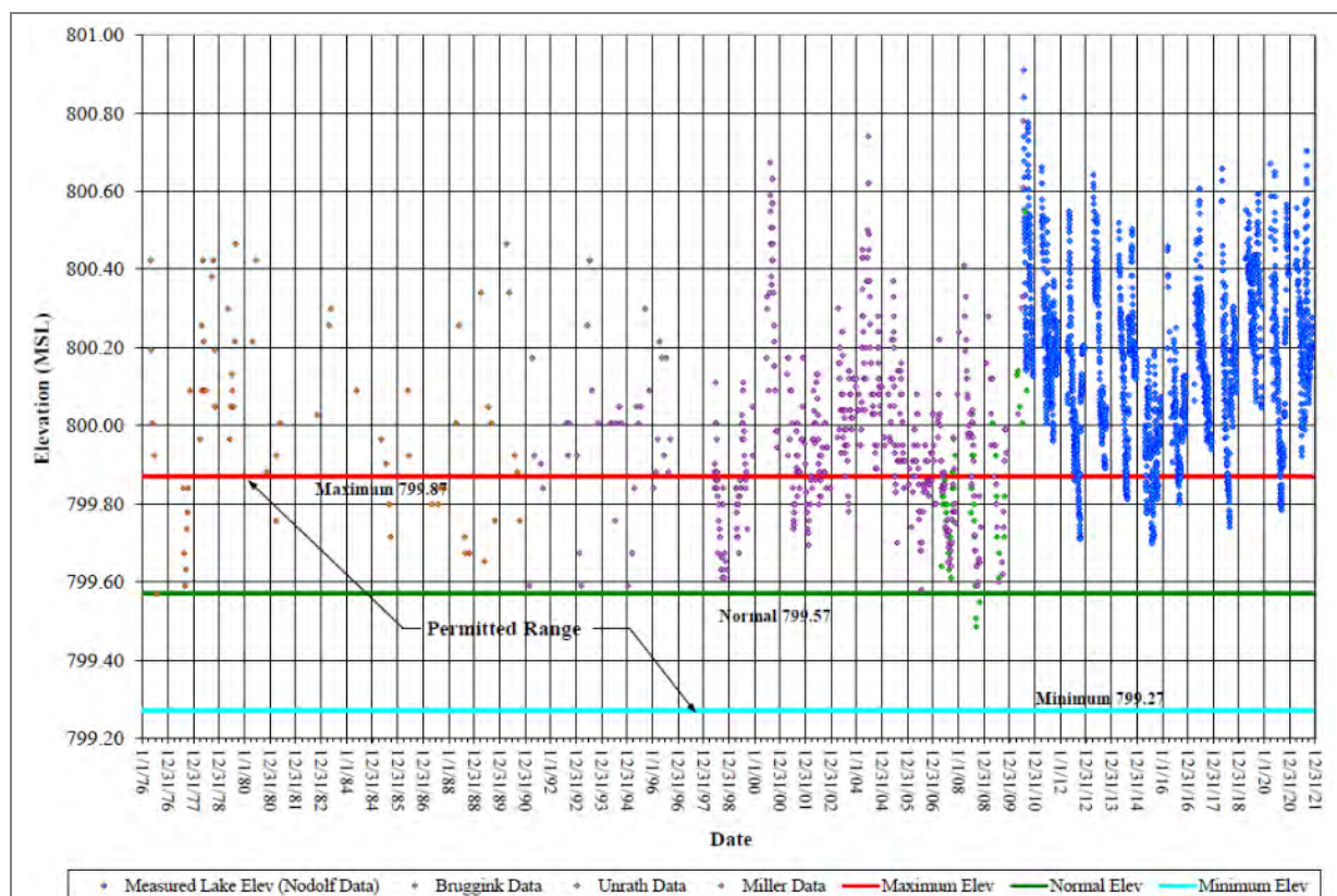
Figure 3.2-1. Cloverleaf Lakes historic lake elevations. Data credit: Denny Nodolf and other volunteers.
