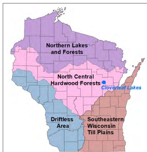
Figure 3.1-2. Location of Cloverleaf Lakes within the ecoregions of Wisconsin. After (Nichols, 1999).
