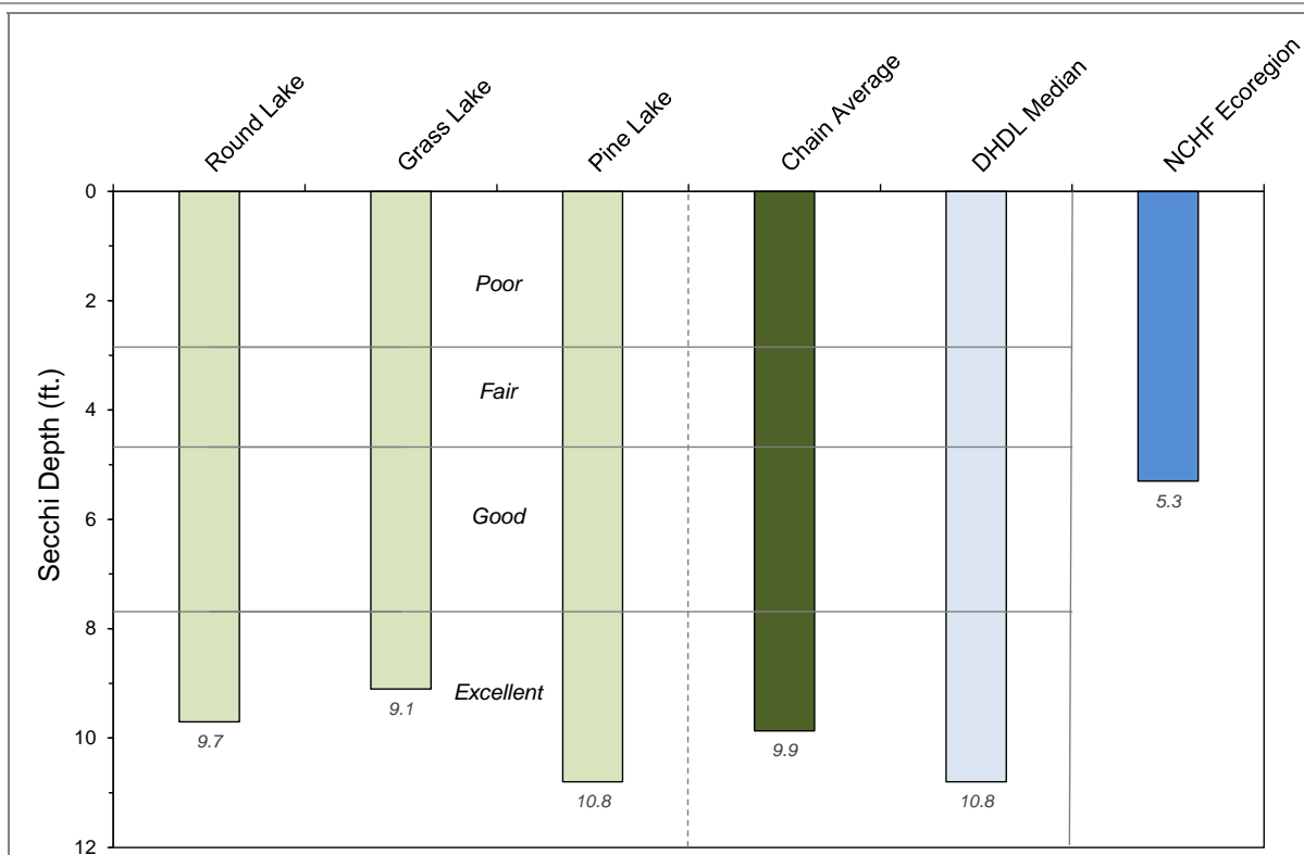
Figure 3.1-7. Cloverleaf Lakes summer average Secchi disk depth and median summer Secchi disk depths from comparable lakes.
